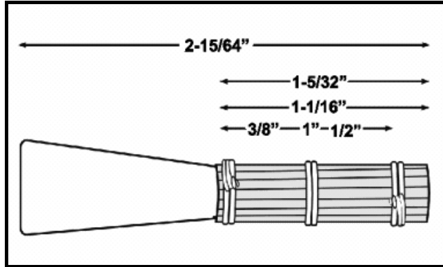
Figure. 1 Bassoon Reed Wire Placement
